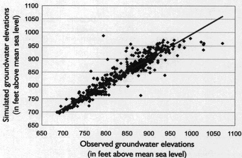
Figure 18. Simulated versus observed groundwater elevations. These results show that the model consistently underestimates the highest measured water levels.
