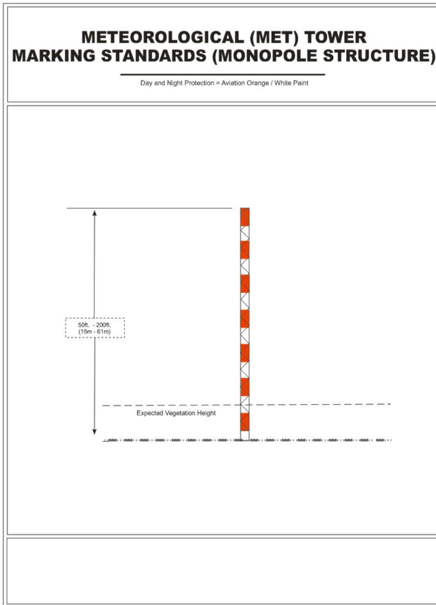
Figure A-1. Meteorological Evaluation Tower (MET) Marking Standards (Monopole Structure)
